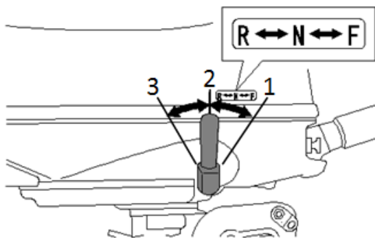
1. Forward position
